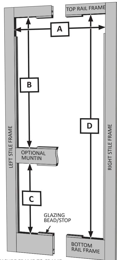
ALUMINUM FRAMED DOOR - EXTERIOR VIEW
